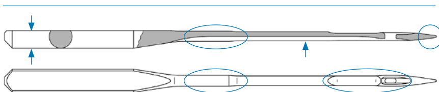
Super Stretch-Nadel
