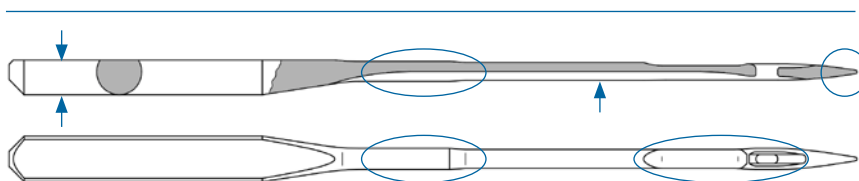
Super Stretch-Nadel
